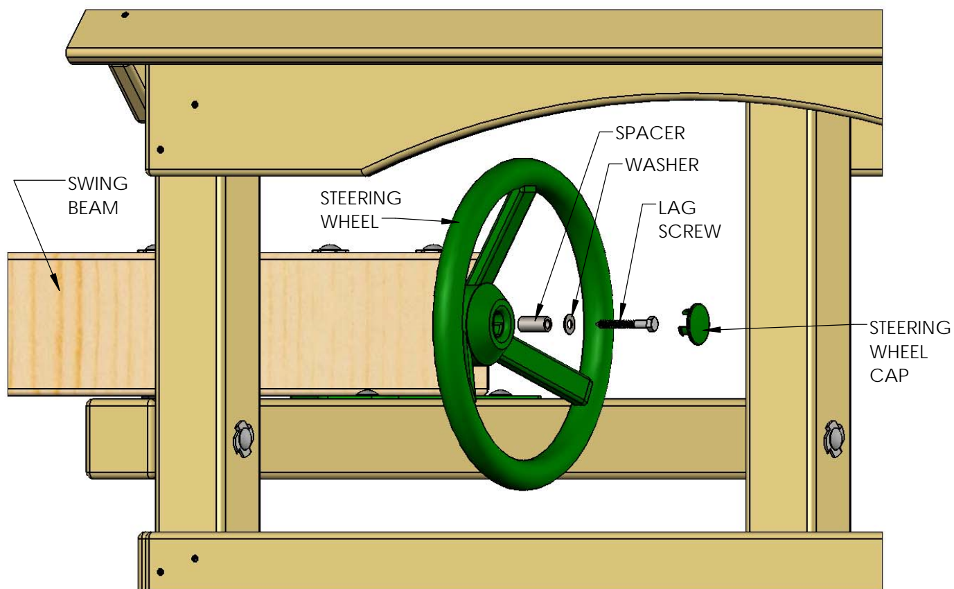
DETAIL A
