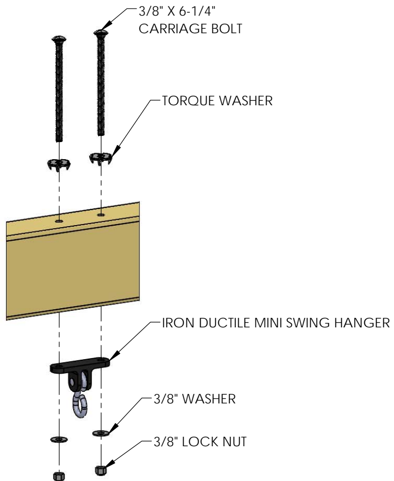
DETAIL A
