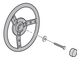
Steering Wheel
