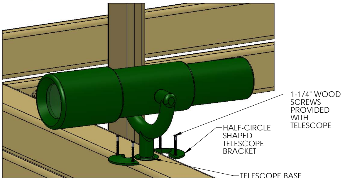
DETAIL A SCALE 1 : 4
