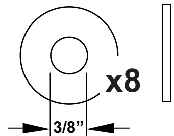
3/8" FLAT WASHER
