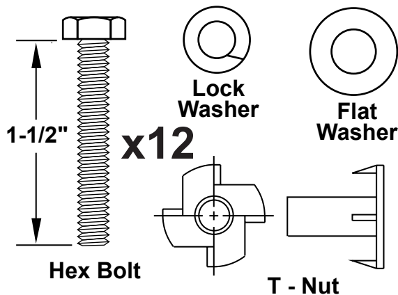
1/4" ROCK WALL HARDWARE
