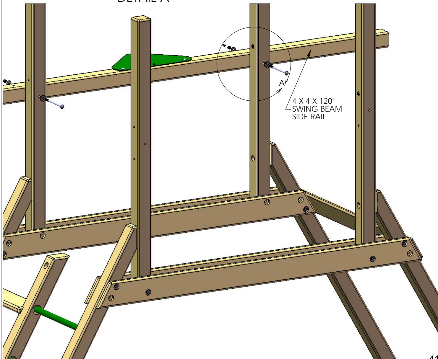
DETAIL A
