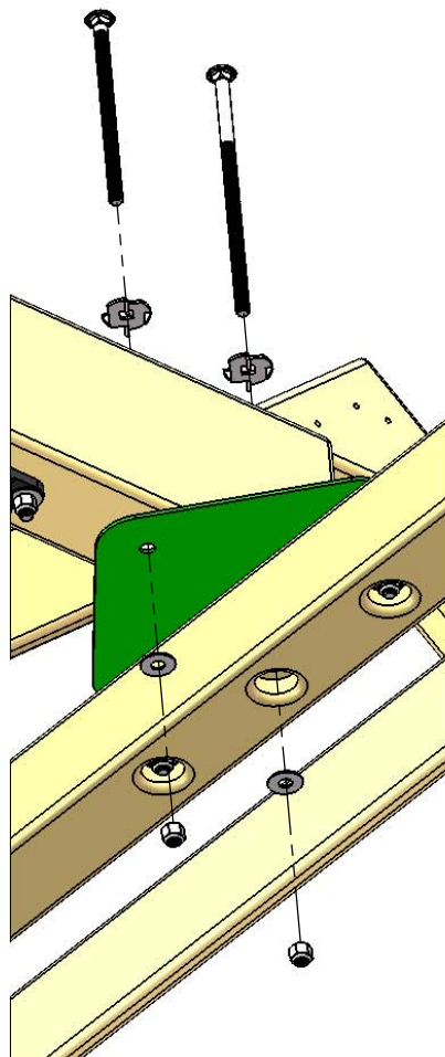
BOTTOM VIEW
