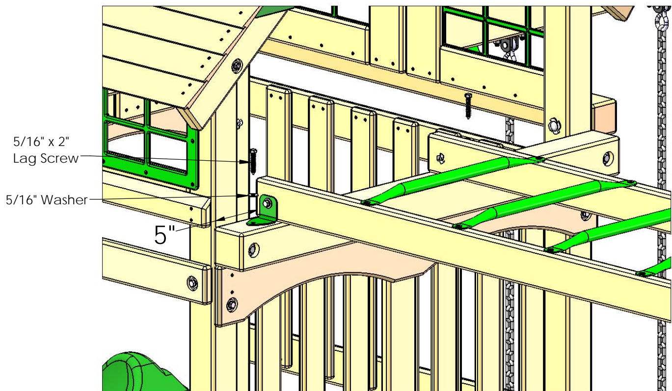
DETAIL A
