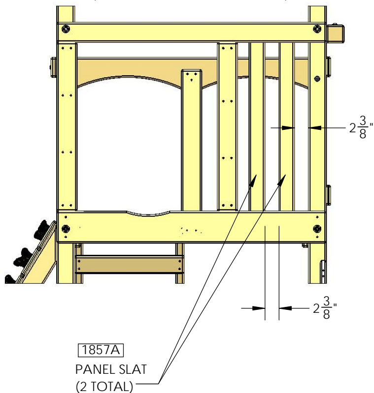
REAR SLAT SPACING (VIEW FROM REAR OF PLAY SET)
