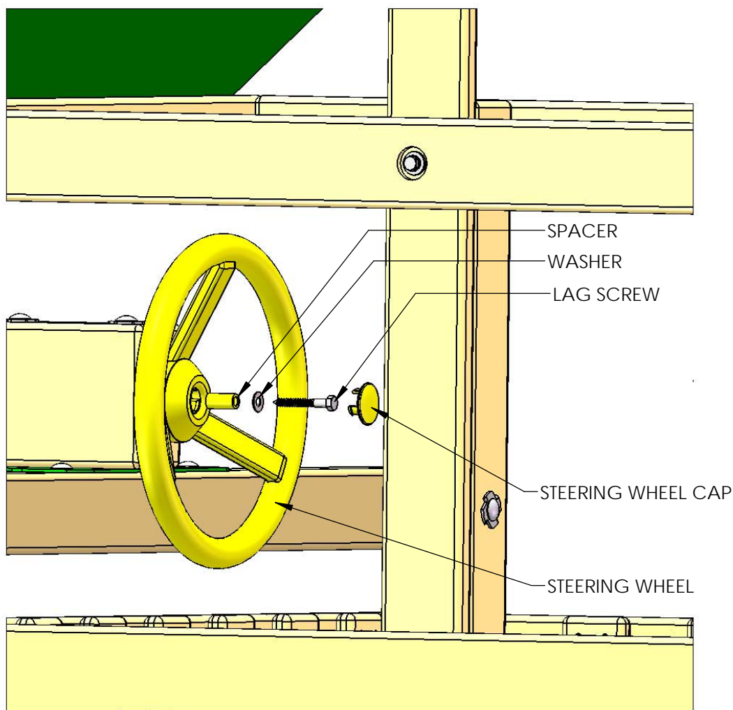
DETAIL A
