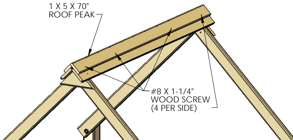
DETAIL A SCALE 1 : 16
