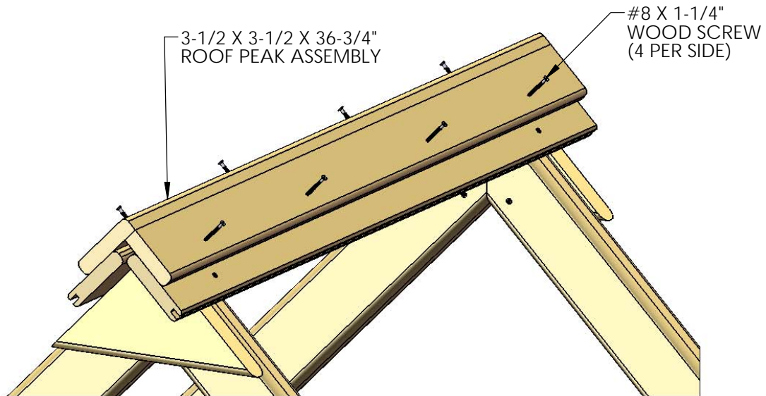
DETAIL A SCALE 1 : 6
