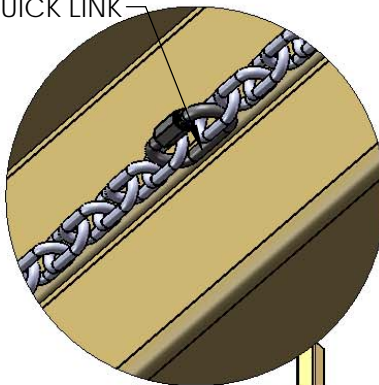
DETAIL B SCALE 1 : 3.5
