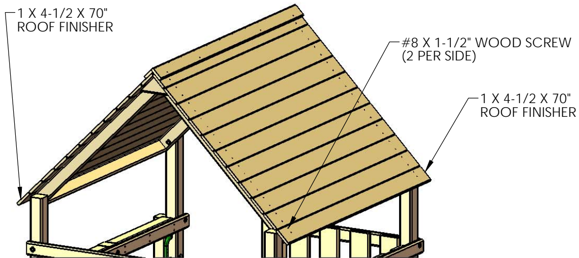
DETAIL A SCALE 1 : 24
