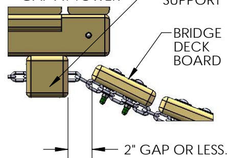
SIDE VIEW OF GAP AT TOWER
