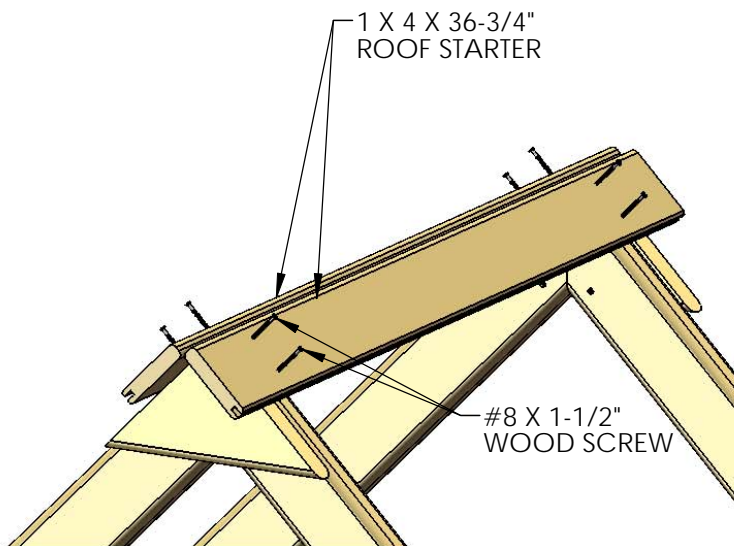
DETAIL B SCALE 1 : 8
